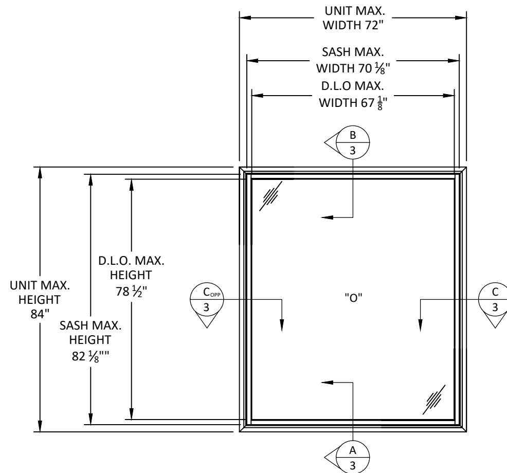
TYPICAL ELEVATION
