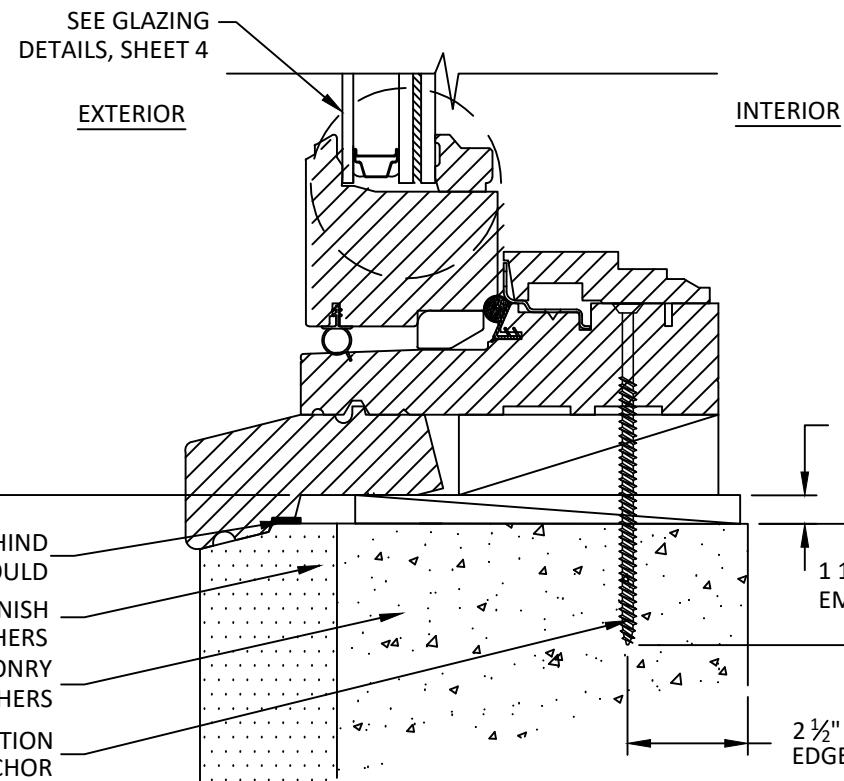
A 3 VERTICAL SECTION SILL - CONCRETE/MASONRY THROUGH FRAME INSTALLATION, TYP.
