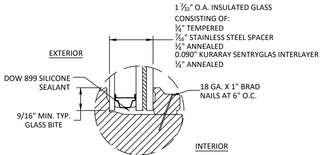
GLAZING DETAIL 3
