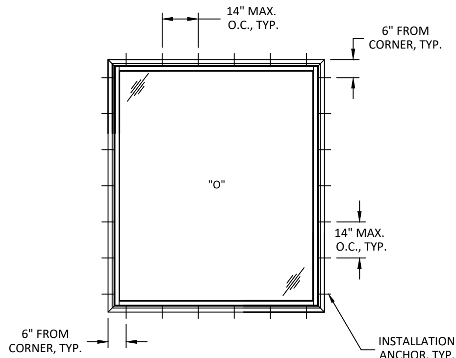
ANCHOR LAYOUT STRAP INSTALLATION
