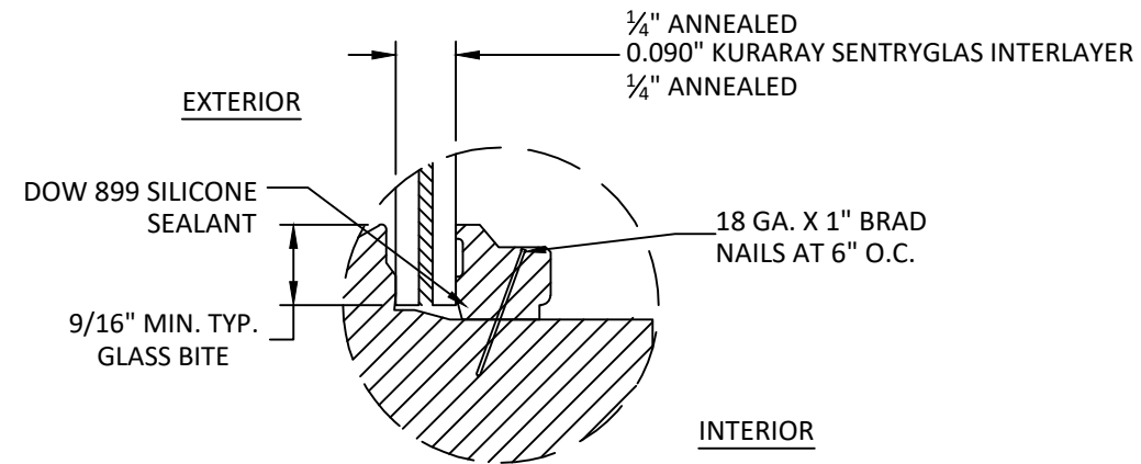
GLAZING DETAIL 4
