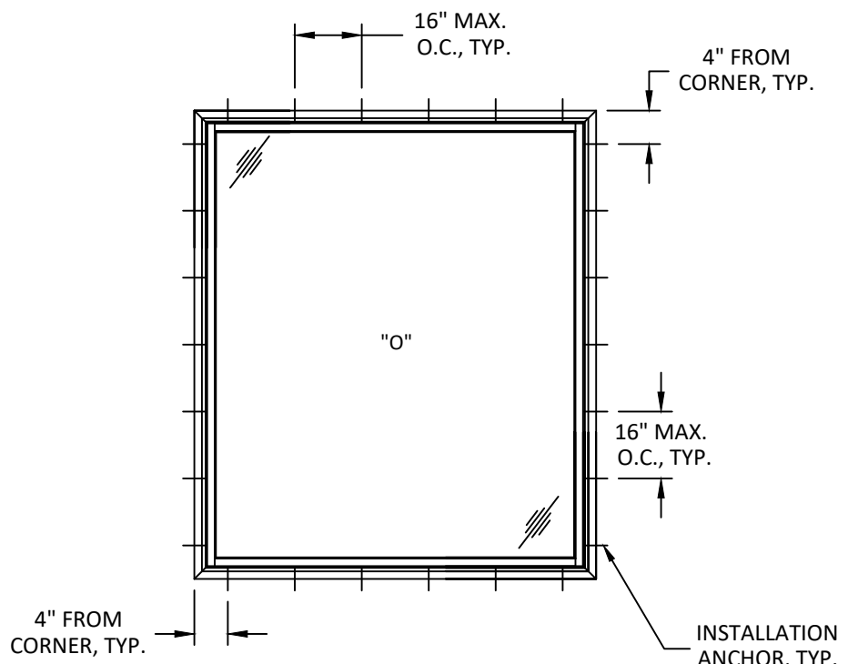
ANCHOR LAYOUT THROUGH FRAME INSTALLATION
