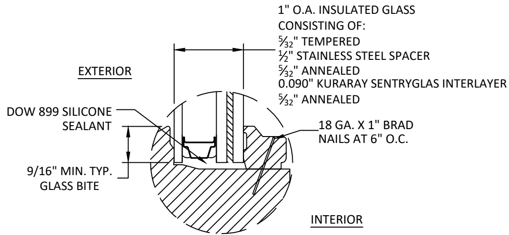
GLAZING DETAIL 1
