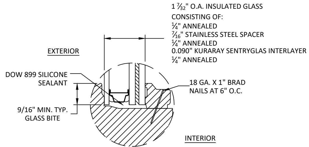
GLAZING DETAIL 2
